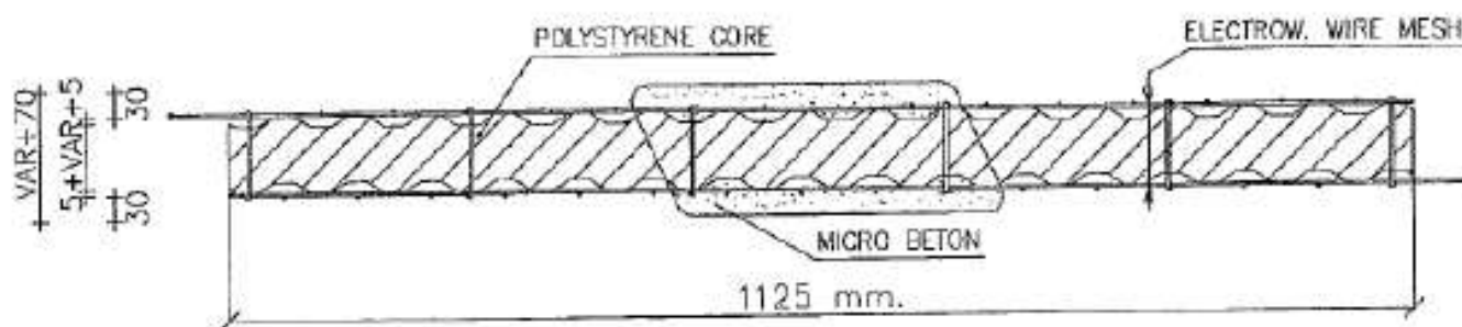
Figure 1: Emedue Single Panel PSM80 Details (Ref. 1, p.7)
