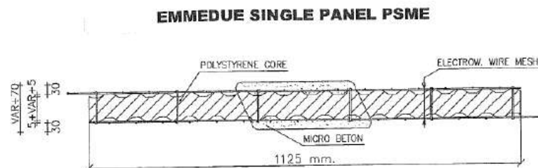
Figure 1: Emmedue Single Panel PSM80 Details (Ref. 1, p.7)
